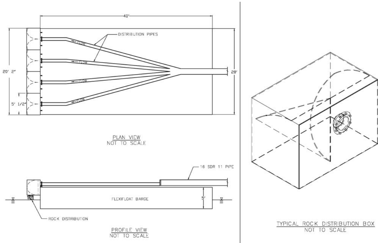
Figure 2. Schematic of the SES Spreader Barge for Armor Stone Placement
